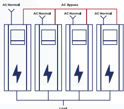
Distributed parallel connection for increased power and redundancy
